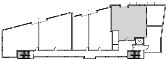
Type G 3 bedroom 2 bathroom +/- 1,390 sqft units 401and 501
